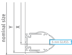
■ Lifting profile with threshold strip and bottom seal
