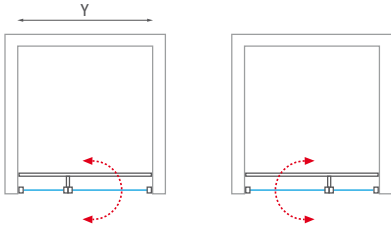
■ BI PF2 + BI SET single shower door to a niche
